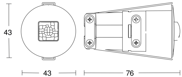
Dimensions (mm)
