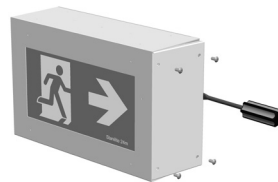
Figure 2: Mains connection and how to get access to main frame
