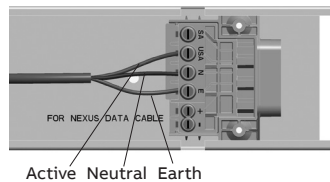
Figure 2: Mains connection and how to get access to main frame
